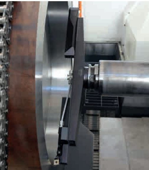
ROUGHING
