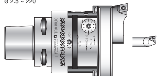
PSC63 - TRM80 Ø 2.5 ~ 220
