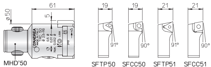
MHD'50
