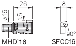
MHD'16
