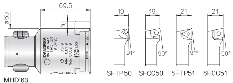
MHD'63
