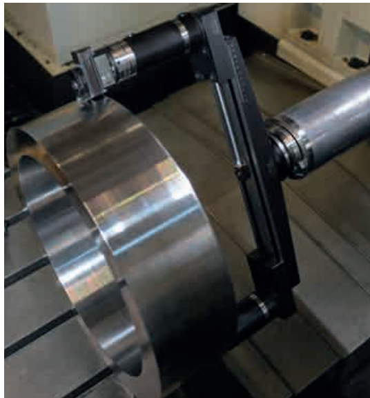
TURNING
